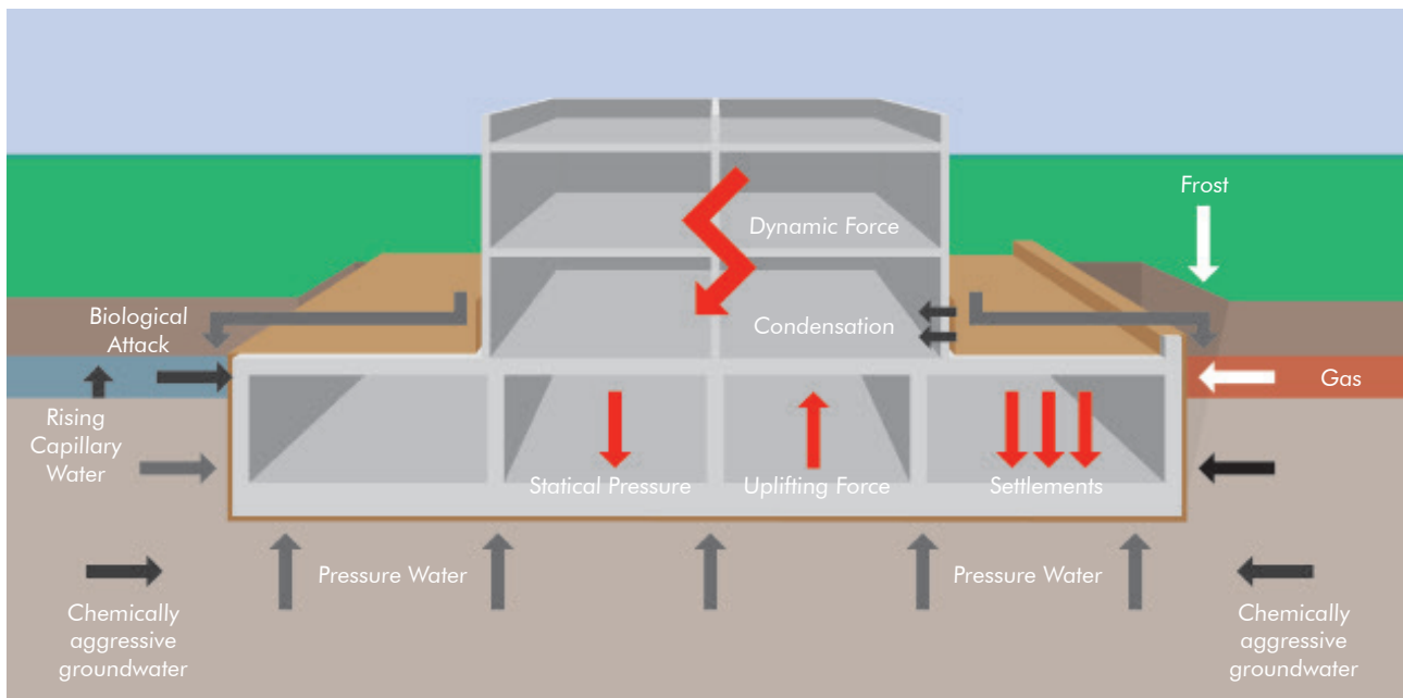
FIGURE 1: Forces Impacting on the Multi Storey Car Park
